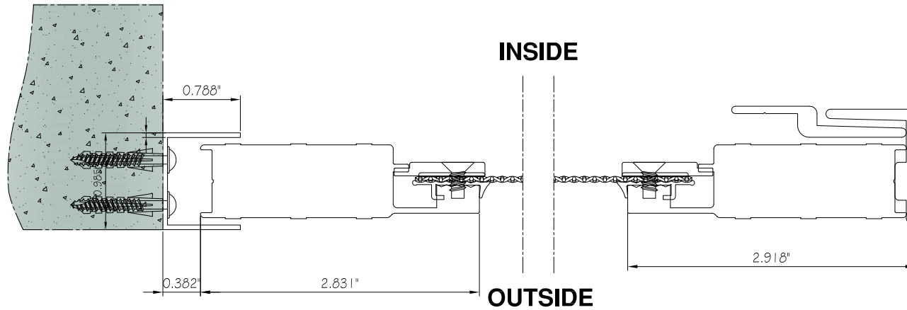
Horizontal cross section
