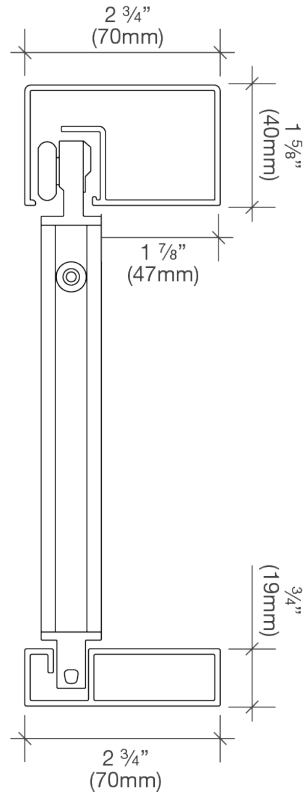
Cross section
