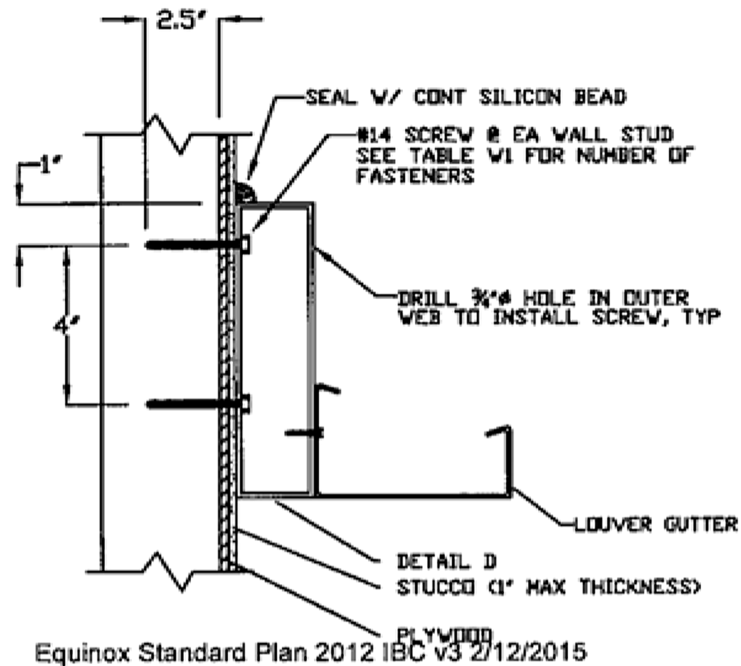
DETAIL J EQUINOX BEAM TO STRUCTURE CONNECTION
