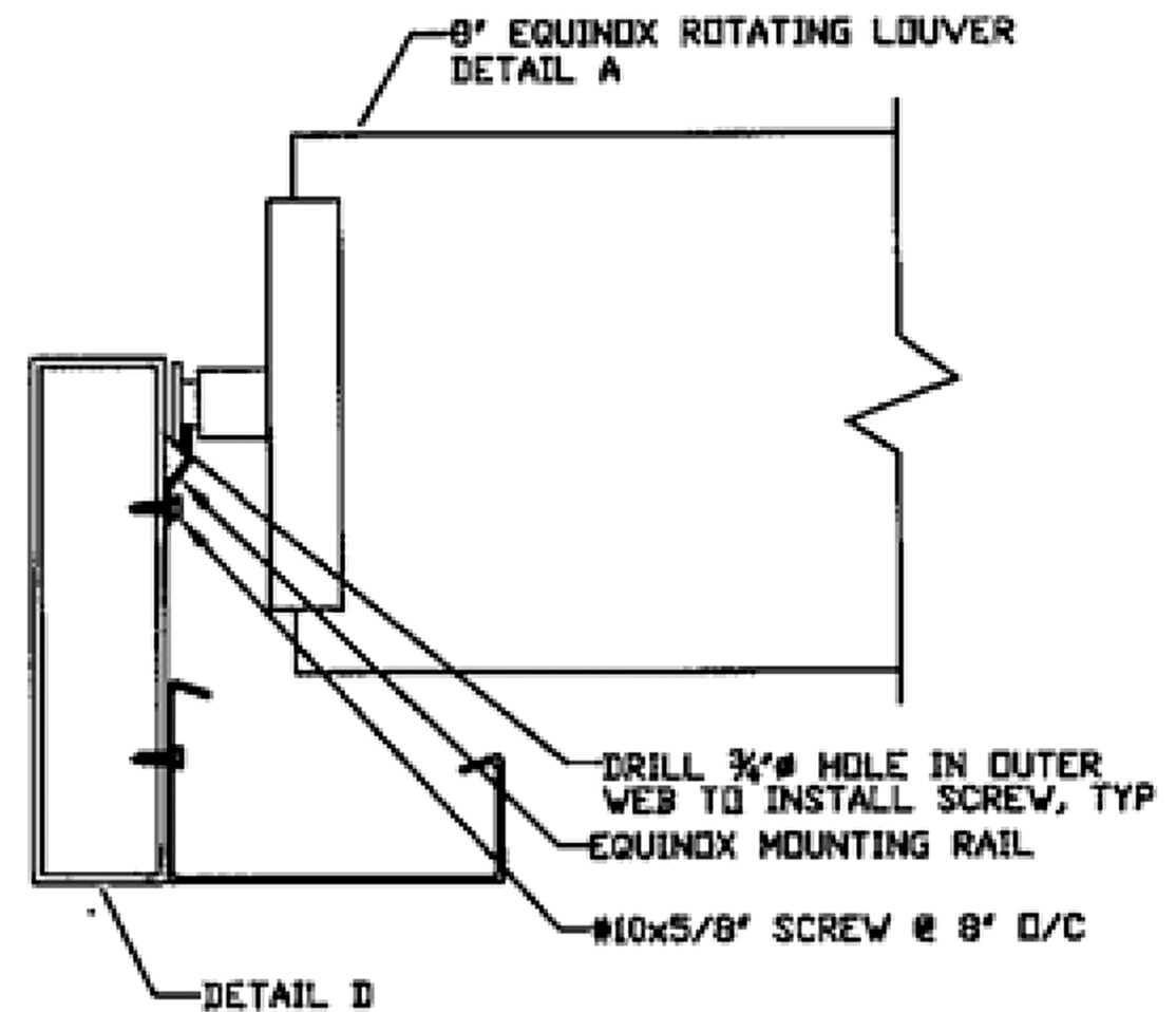
DETAIL H EQUINOX LOUVER TO MOUNTING RAIL TO HEADER CONNECTION
